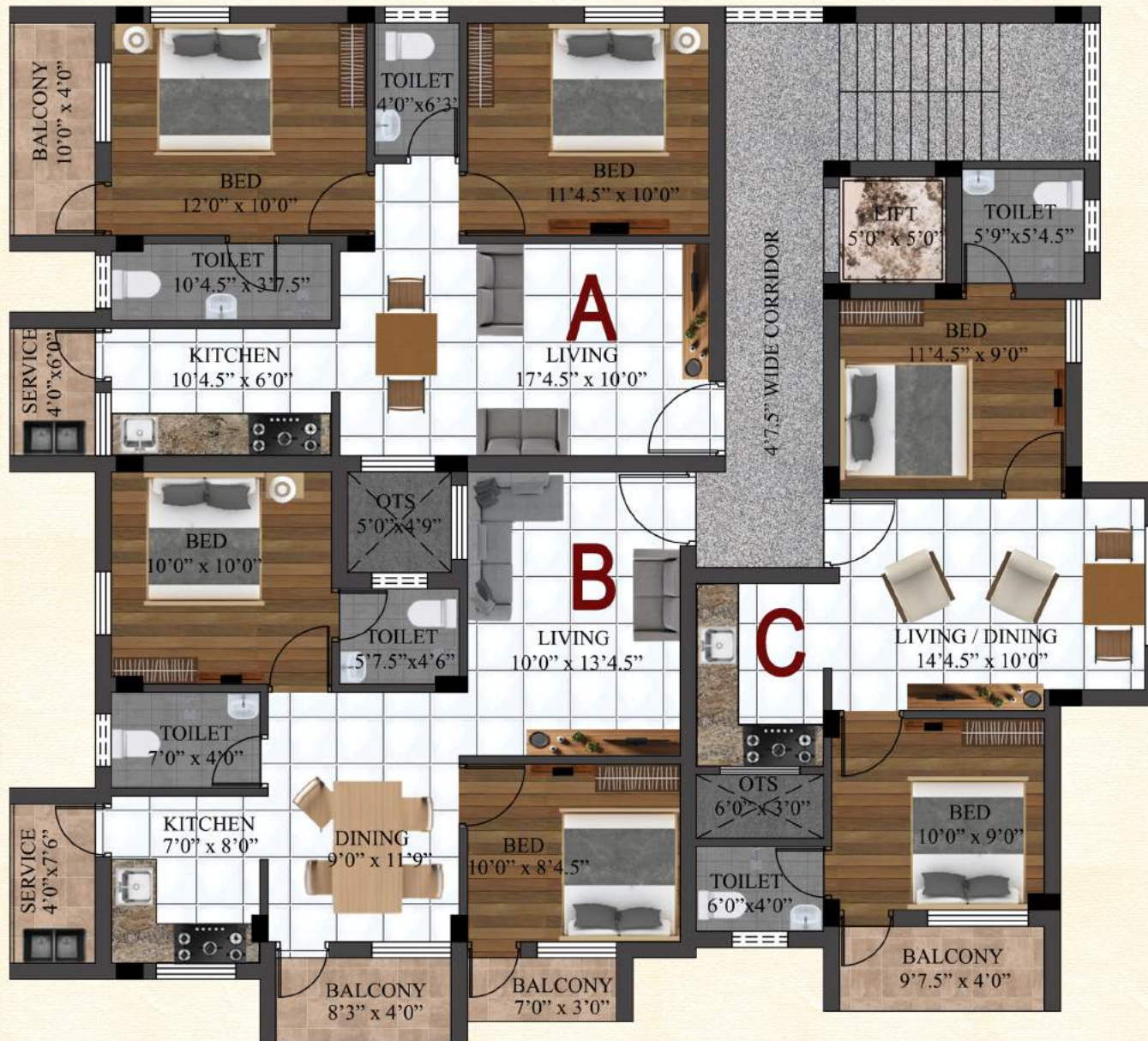
2 nd , 3 rd and 4 th FLOOR PLAN
